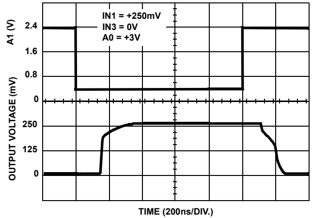
FIGURE 4. CHANNEL-TO-CROSSING SWITCHING RESPONSE
