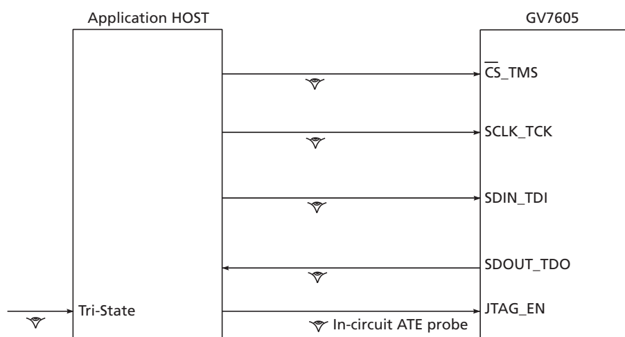
Figure 4-66: System JTAG
