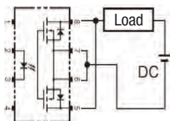
DIP 8-pin package (for □CR□/□FR□ types only)
