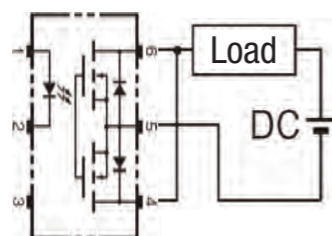
DIP/SOP 6-pin package
