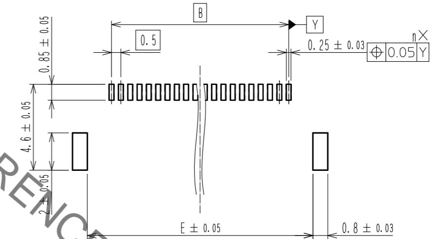
RECOMMENDED STENCIL PATTERN (RECOMMENDED STENCIL THICKNESS : t=0.12 )
