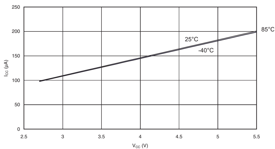
Figure 184. AREF External Reference Current vs. V_{CC}
