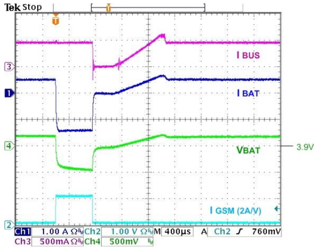
Figure 23. GSM Pulse (2 A Step, t_R/t_F=5\ \mu\text{s} ) Response, 3.9 V BAT , 1 k \Omega LDO Load, I BUSLIM =500 mA, I CHRG =1.0 A
