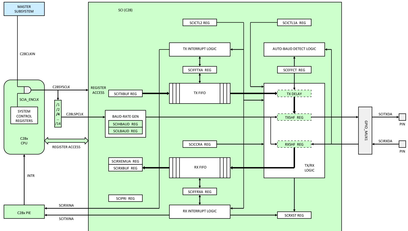
Figure 5-50. SCI (C28x)
