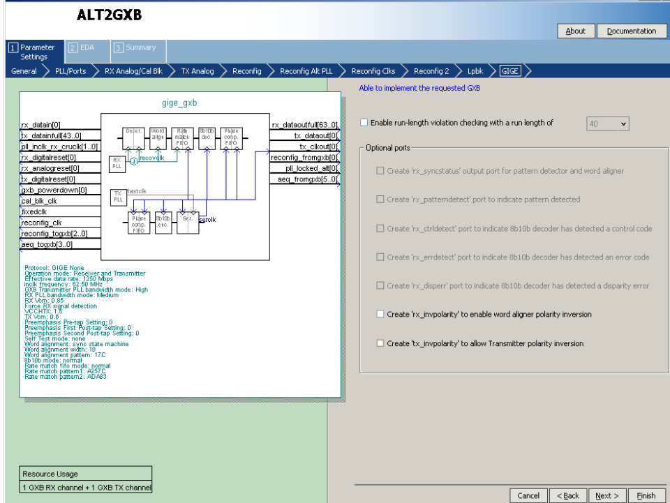
MegaWizard Plug-In Manager [page 12 of 14]
