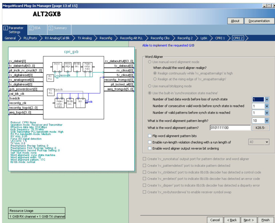
Figure 4–81. MegaWizard Plug-In Manager - ALT2GX (CPRI 2)
