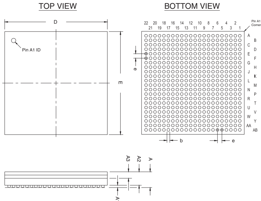
Figure 10–1. 484-Pin FBGA Package Outline
