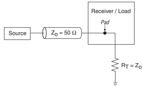
Figure 11–23. Simple Parallel Fly-By Termination
