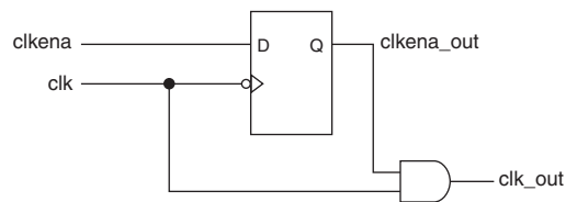
Figure 1–55. clkena Implementation
