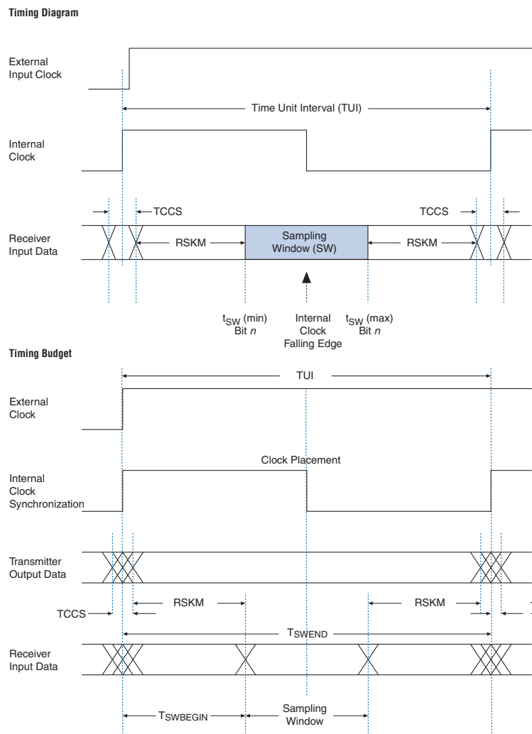
Figure 5–19. Differential High-Speed Timing Diagram and Timing Budget for Non-DPA
