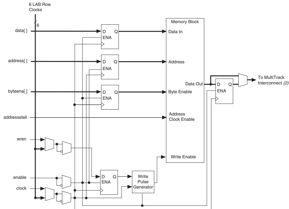
Figure 2–19. Stratix II and Stratix II GX Single-Clock Mode in Single-Port Mode Note (1)
