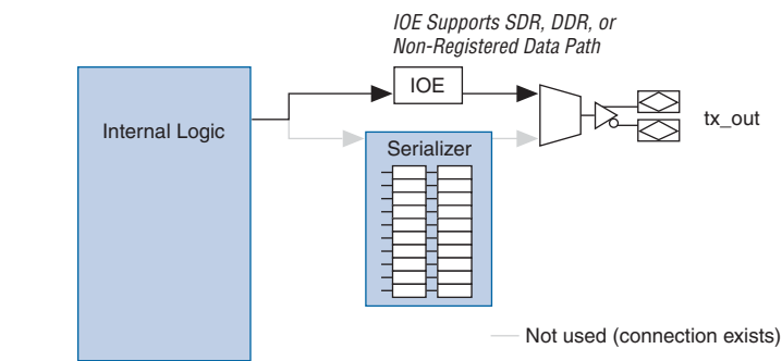
Figure 5-5. Serializer Bypass
