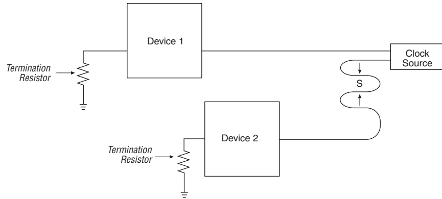
Figure 11–20. Serpentine Routing
