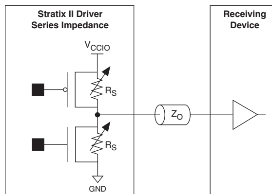
Figure 4-24. Stratix II and Stratix II GX On-Chip Series Termination with Calibration
