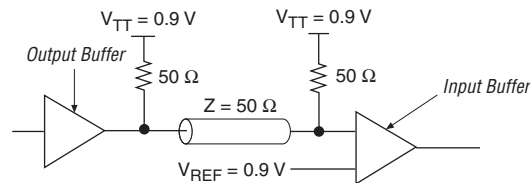
Figure 4–6. 1.8-V HSTL Class II Termination
