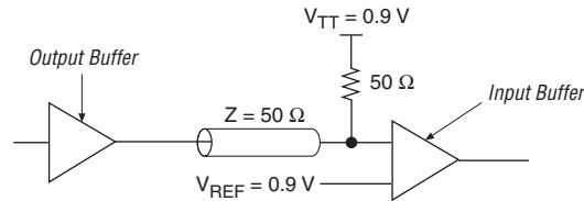
Figure 4–5. 1.8-V HSTL Class I Termination
