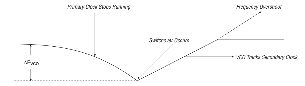
Figure 1–25. VCO Switchover Operating Frequency
