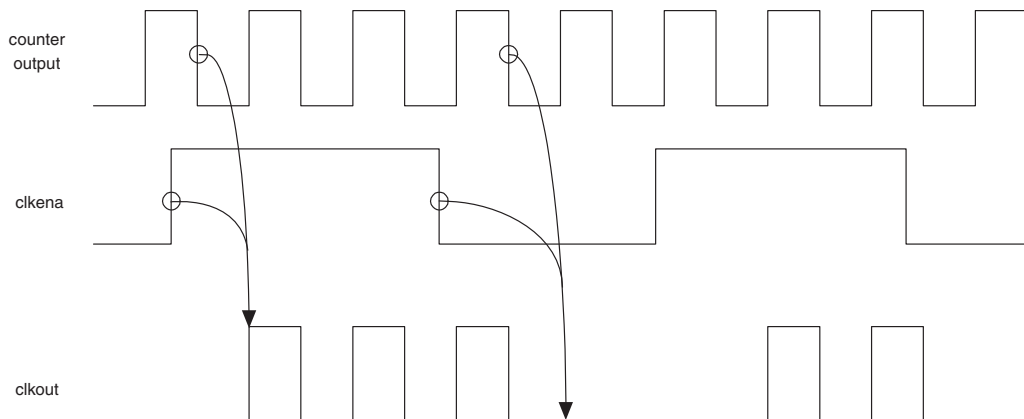
Figure 1–56. Clkena Signals
