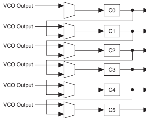
Figure 1–16. Counter Cascading
