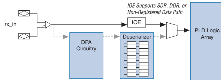
Figure 5-7. Deserializer Bypass
