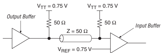
Figure 4–8. 1.5-V HSTL Class II Termination
