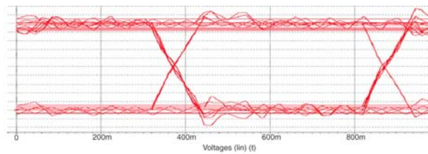
Figure 11–16. Stub Length = 0.25 Inch
