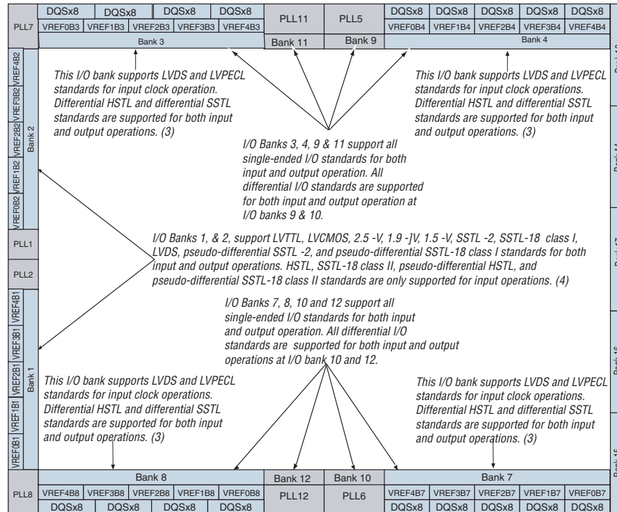
Figure 4–22. Stratix II GX I/O Banks Notes (1), (2), (3), (4)
