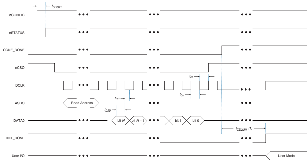
Figure 7-16. AS Configuration Timing
