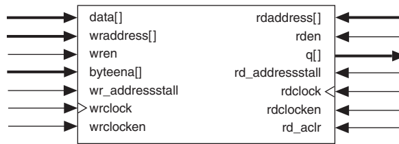
Figure 2–7. Stratix II and Stratix II GX Simple Dual-Port Memory Note (1)
