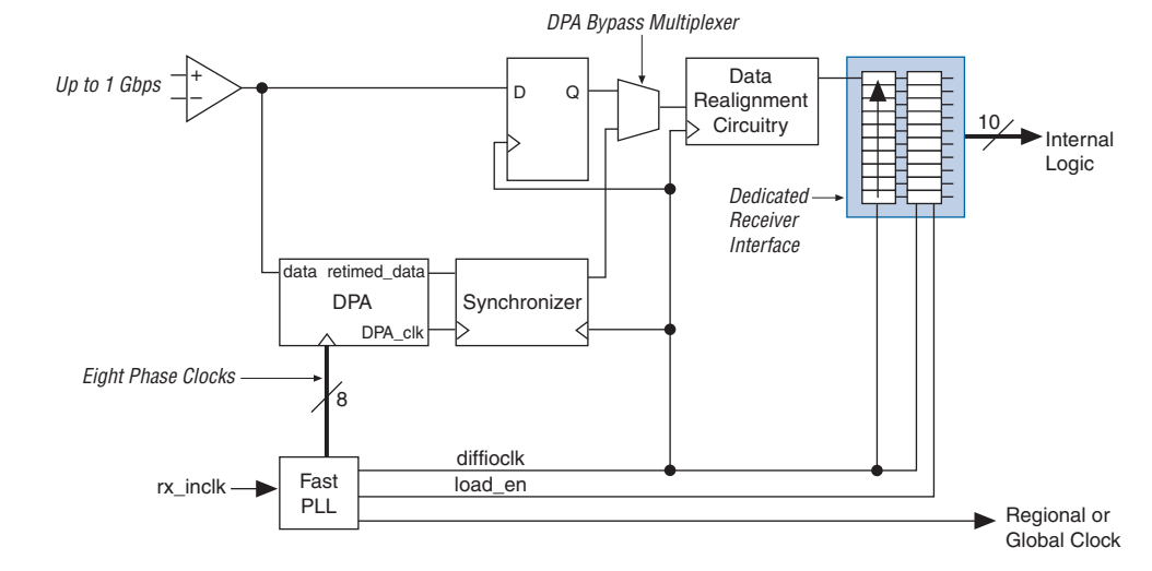
Figure 5–6. Receiver Block Diagram
