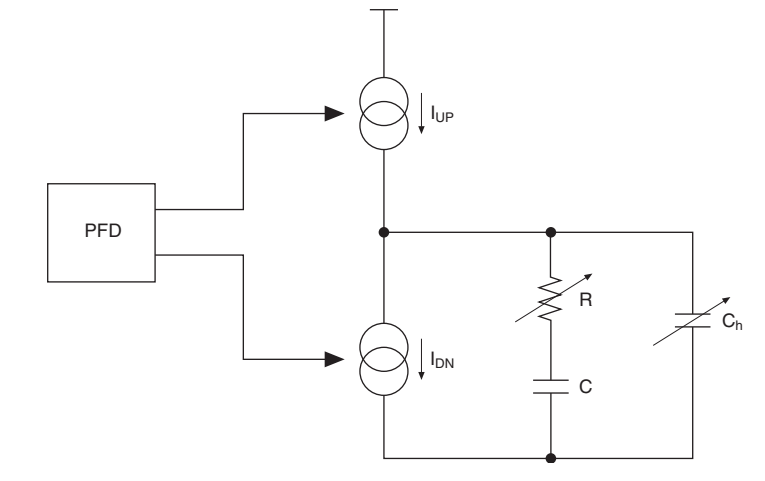
Figure 1–31. Loop Filter Programmable Components
