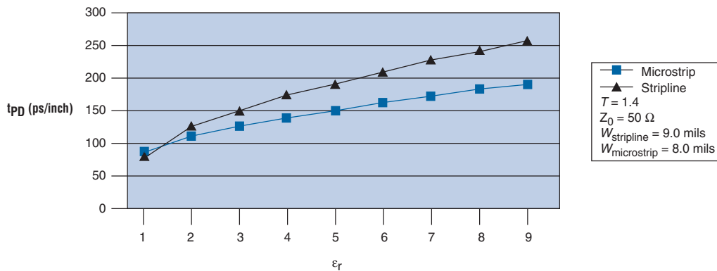
Figure 11–9. Propagation Delay Versus Dielectric Constant for Microstrip & Stripline Traces
