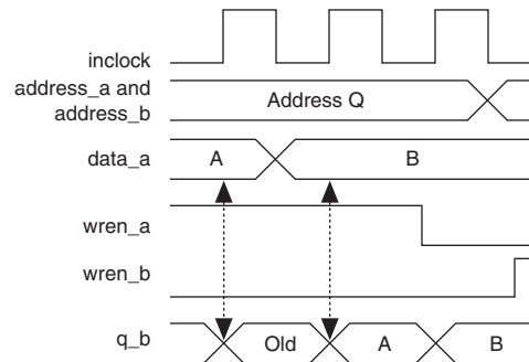
Figure 2–22. Stratix II and Stratix II GX Mixed-Port Read-During-Write: OLD_DATA
