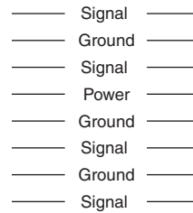
Figure 11–36. Example Eight-Layer Stack-Up
