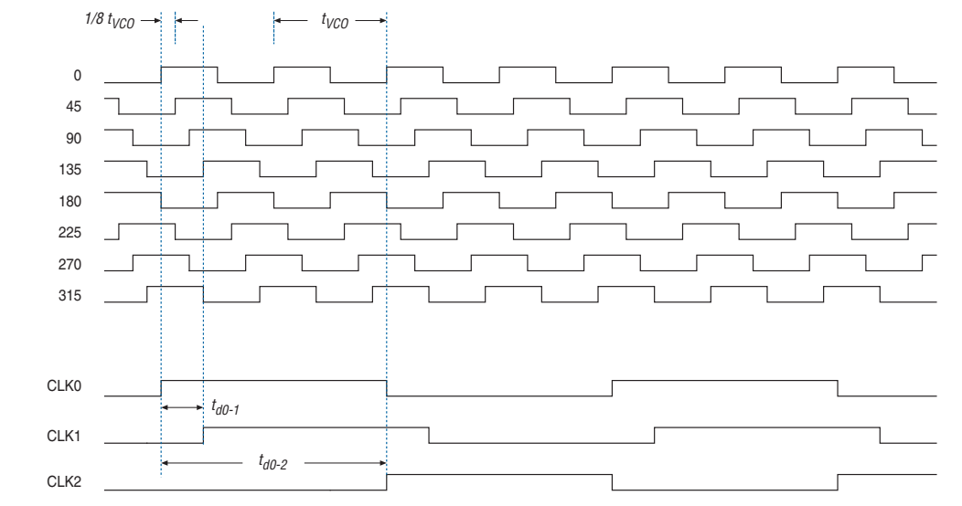
Figure 1–14. Delay Insertion Using VCO Phase Output and Counter Delay Time
