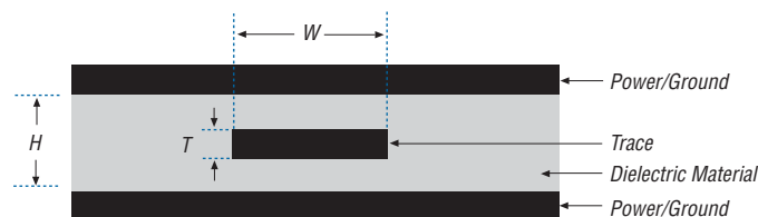
Figure 11–2. Stripline Transmission Line Layout Note (1)
