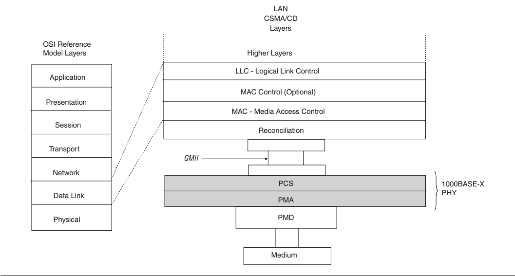
Figure 6–1. GMII Position Relative to OSI Reference Model
