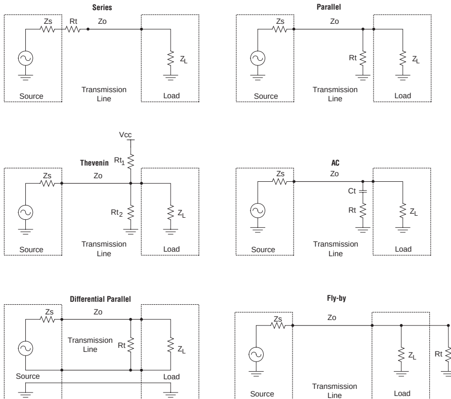
Figure 4–54. Termination Techniques
