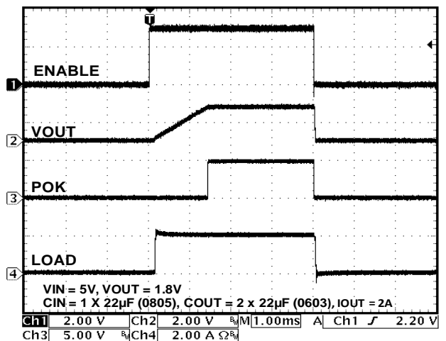
Startup Waveforms at 2A
