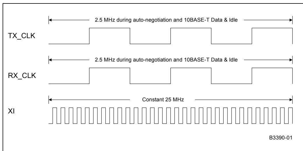
Figure 10 Clocking for 10BASE-T
