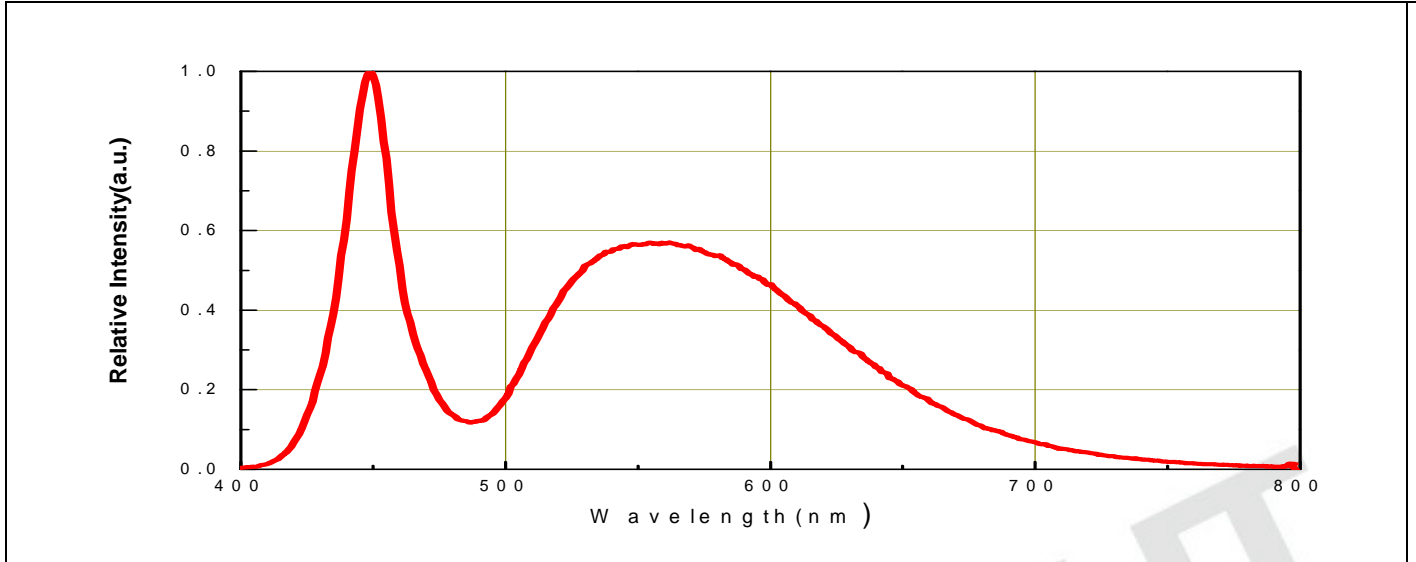
Relative Spectral Distribution, I_F=500\text{mA}@50\text{ms} , T_{\text{solder pad}}=25
