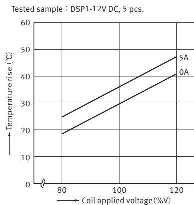
3.-(2) Coil temperature rise (1 Form A 1 Form B)
