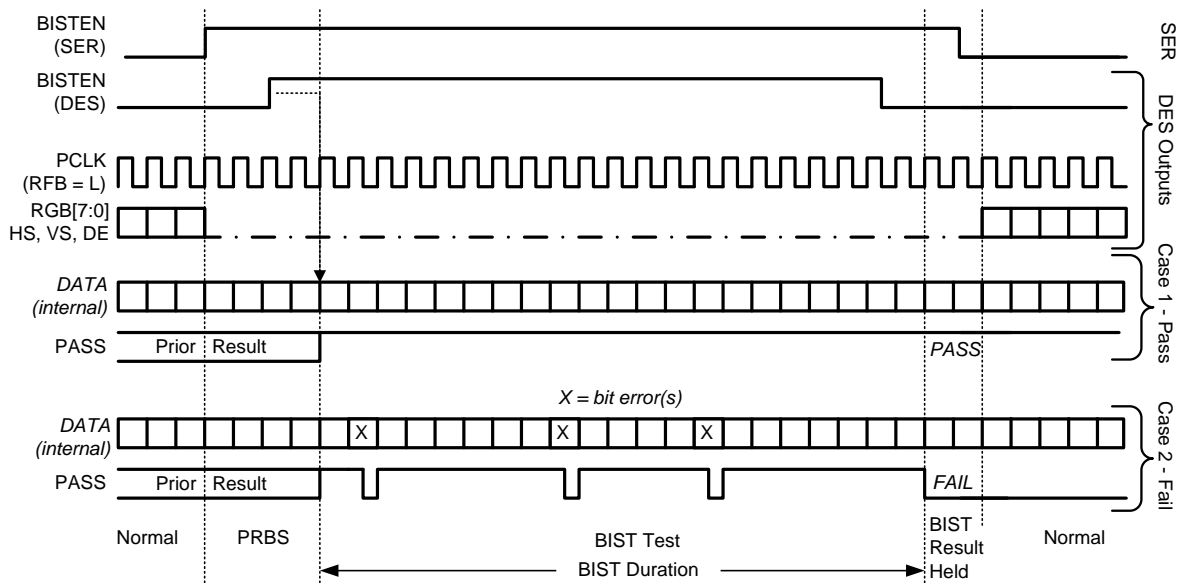
Figure 33. BIST Waveforms
