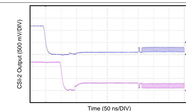
Figure 18. CSI-2 D0± Start of Transmission
