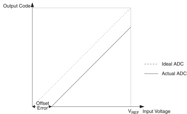
Figure 21-10. Offset Error
