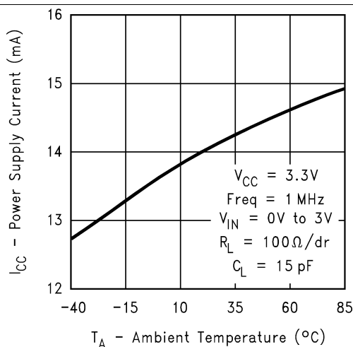
Figure 8. Power Supply Current vs Ambient Temperature
