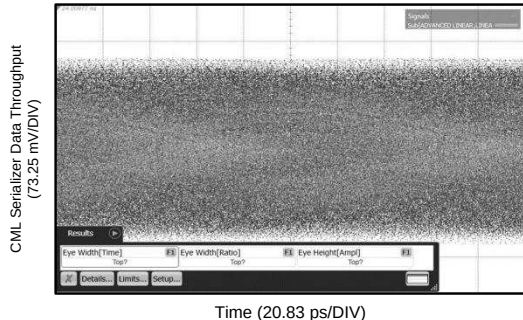
Figure 17. TL = 5-Meter 30-AWG 100 \Omega Twin-Axial Cable, No Repeater, 8 Gbps
