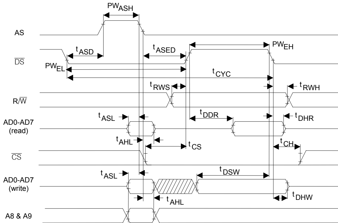
Figure 19-3. Motorola Bus Timing (BTS = 1 / BIS[1:0] = 00)
