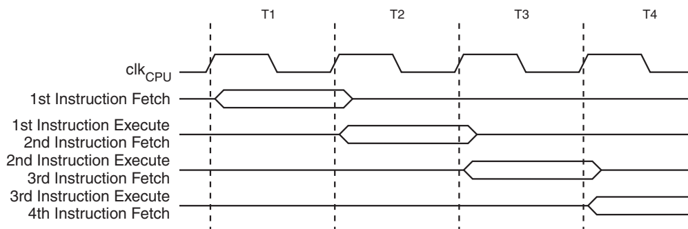
Figure 1. The Parallel Instruction Fetches and Instruction Executions
