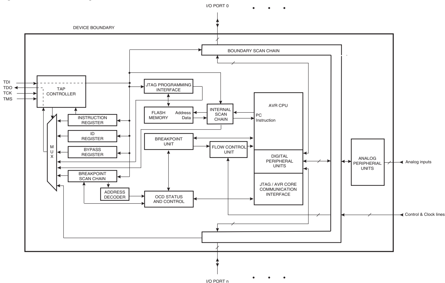
Figure 22-1. Block Diagram
