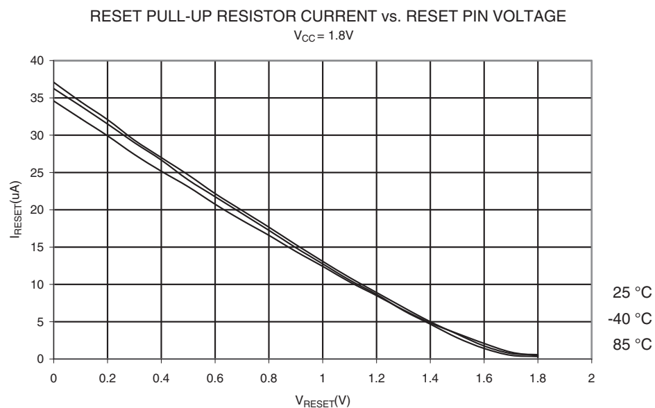
Figure 27-16. Reset Pull-up Resistor Current vs. Reset Pin Voltage ( V_{CC} = 1.8\text{ V} )
