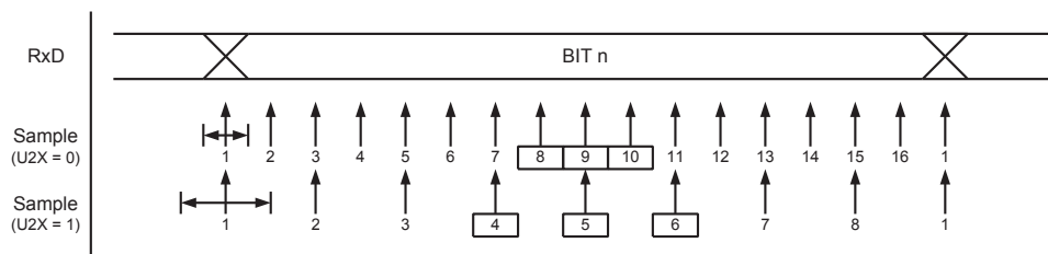
Figure 18-7. Sampling of Data and Parity Bit
