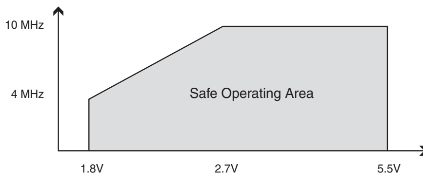
Figure 26-1. Maximum Frequency vs. V_{CC} (4 - 10 MHz).
