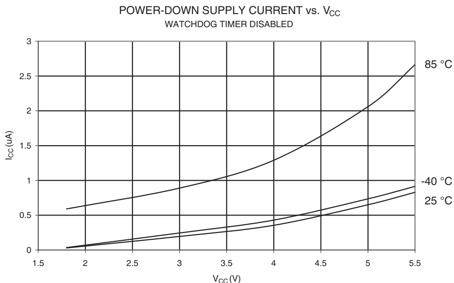
Figure 27-9. Power-down Supply Current vs. V_{CC} (Watchdog Timer Disabled)
