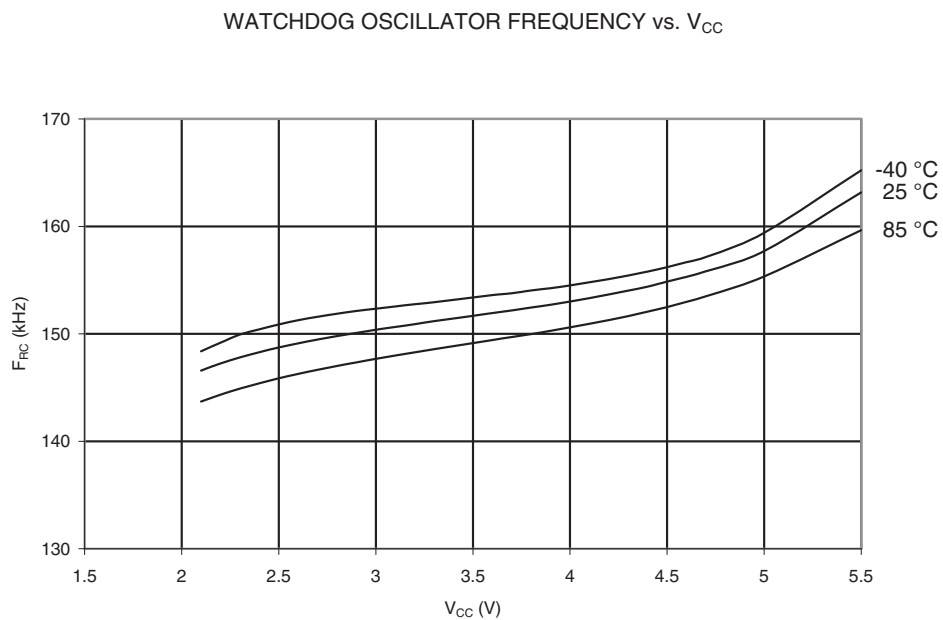
Figure 27-40. Watchdog Oscillator Frequency vs. V_{CC}
