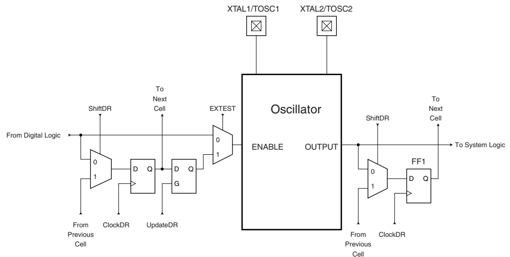
Figure 23-5. Boundary-scan Cells for Oscillators and Clock Options
