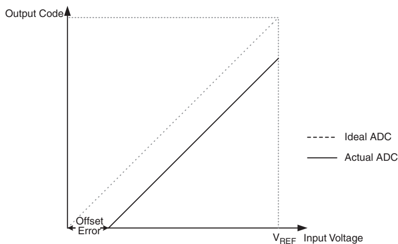
Figure 21-10. Offset Error
