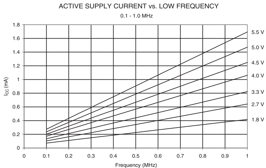
Figure 27-1. Active Supply Current vs. Low Frequency (0.1 - 1.0 MHz)
