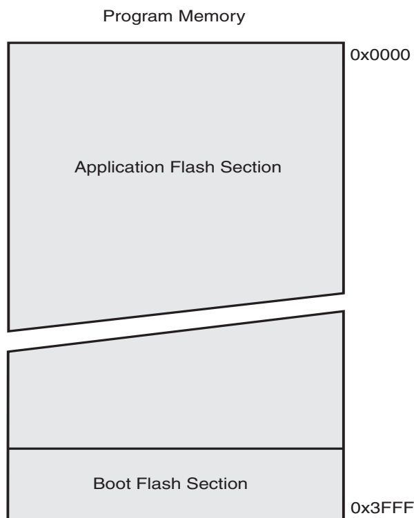
Figure 7-1. Program Memory Map
