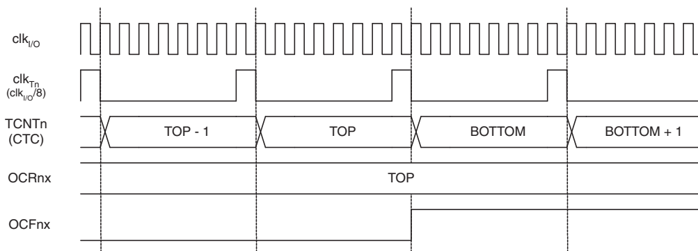
Figure 7. Timer/Counter Timing Diagram, Clear Timer on Compare Match mode, with Prescaler ( f_{clk\_I/O}/8 )
