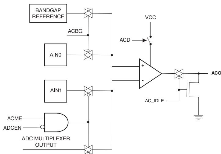
Figure 23-6. Analog Comparator
