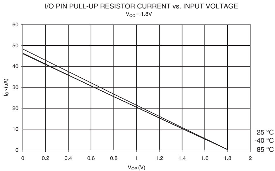
Figure 27-13. I/O Pin Pull-up Resistor Current vs. Input Voltage ( V_{CC} = 1.8 V)
