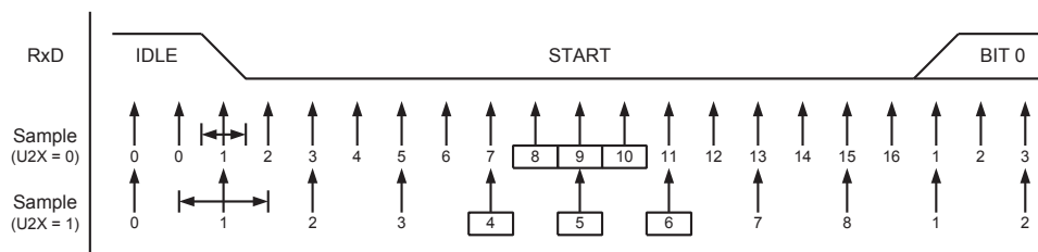
Figure 18-6. Start Bit Sampling
