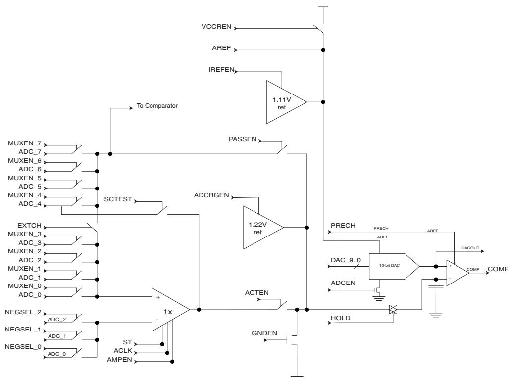
Figure 23-8. Analog to Digital Converter
