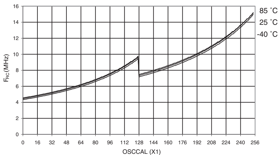
Figure 26-85. Calibrated 8 MHz RC Oscillator vs. OSCCAL Value
