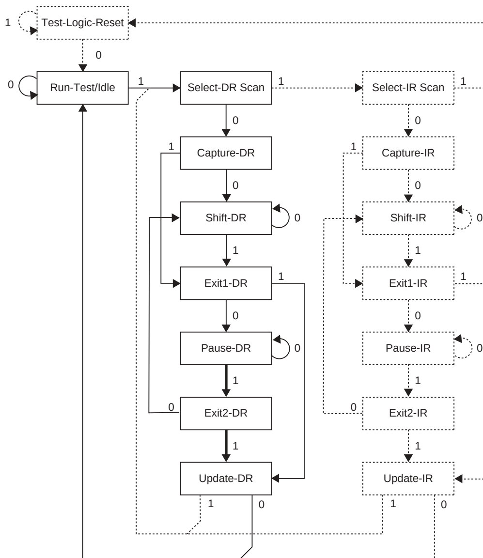
Figure 103. State Machine Sequence for Changing / Reading the Data Word
