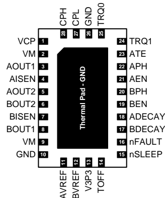
RHR Package 28-Pin WQFN Top View DRV8881E
