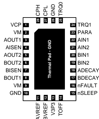
RHR Package 28-Pin WQFN Top View DRV8881P
