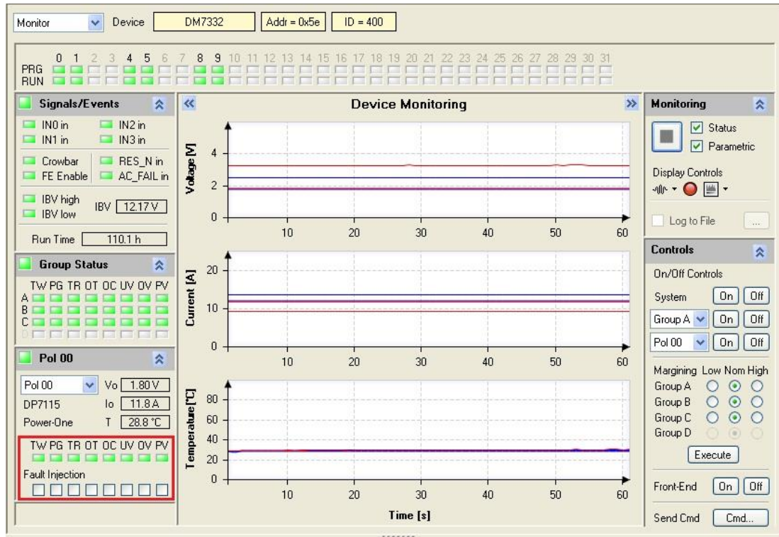
Figure 51. Fault Injection Controls In Monitor Window
