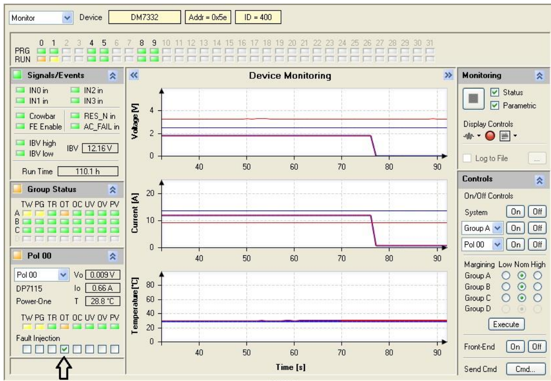
Figure 52. Example Overtemp Fault Injection in the GUI
