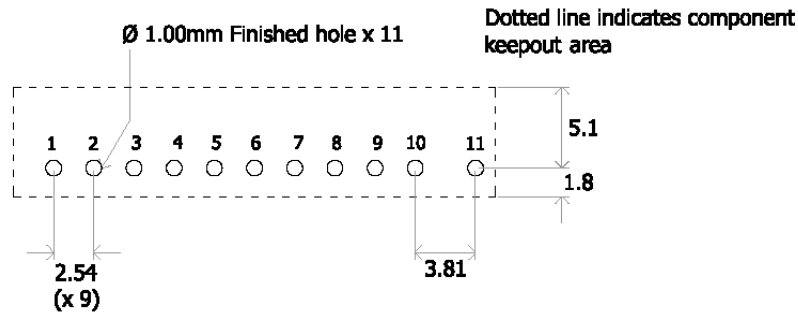
Figure 56 - Recommended Footprint – Top View
