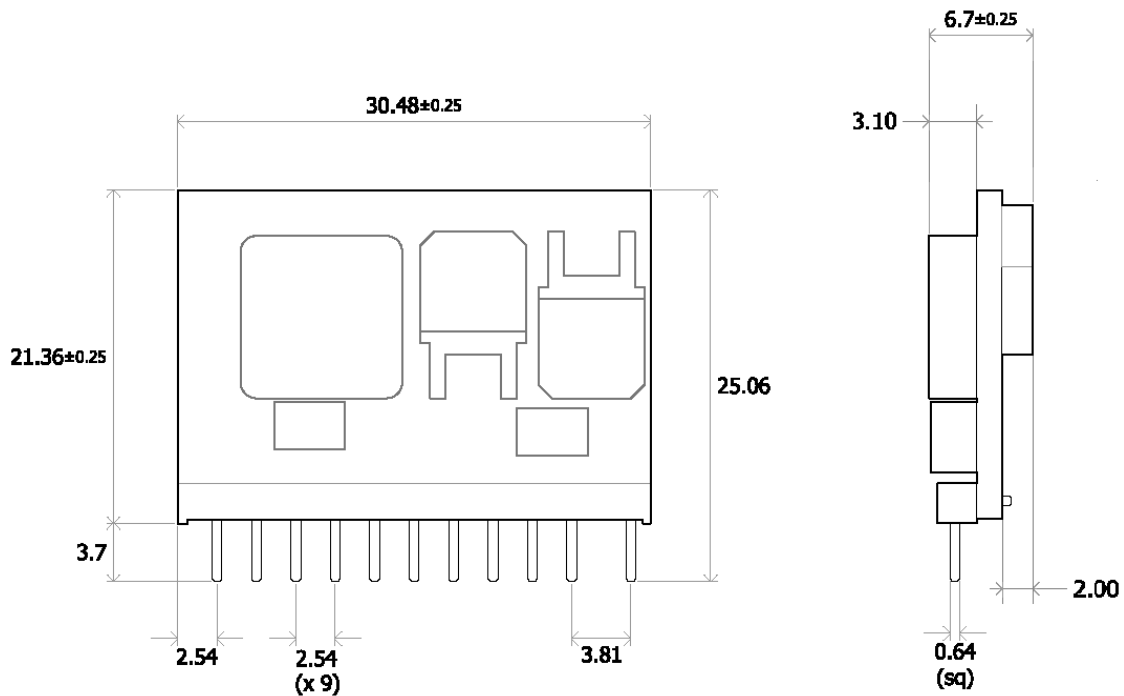
Figure 55 - Mechanical Drawing
