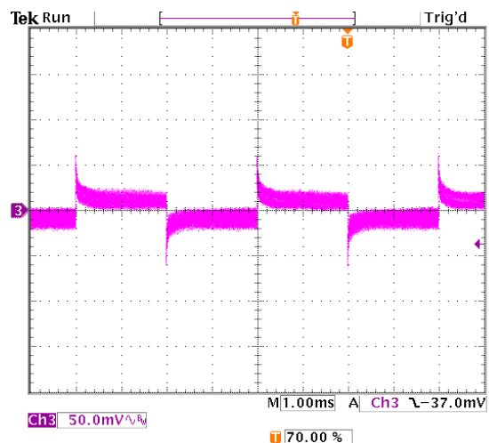
Figure 48. Transient Response with Regulation set to 3.72 mV/A.
