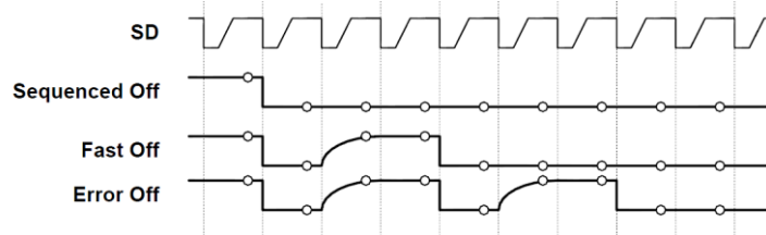
Figure 39. OK Severity Encoding Waveforms
