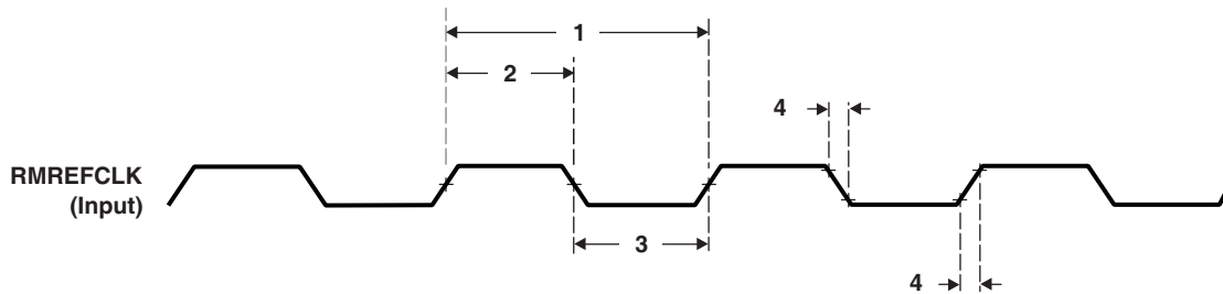
Figure 8-14. RMREFCLK Timing RMI Operation
