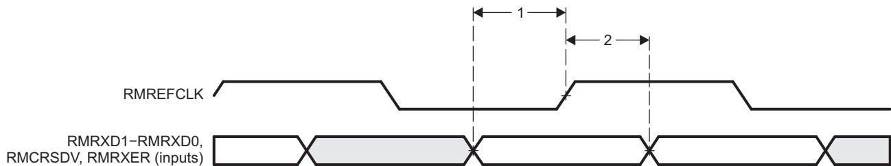
Figure 8-15. EMAC Receive Interface Timing RMI Operation
