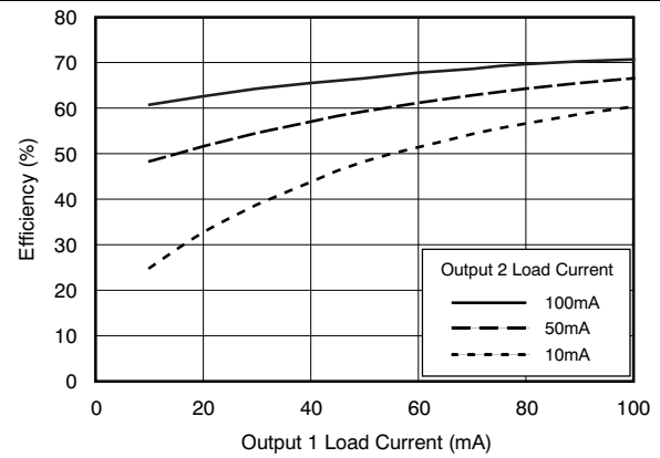
Figure 2. DCH010505D Efficiency
