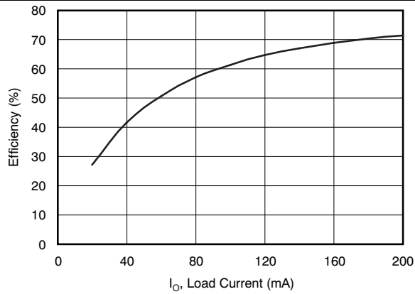
Figure 1. DCH010505S Efficiency
