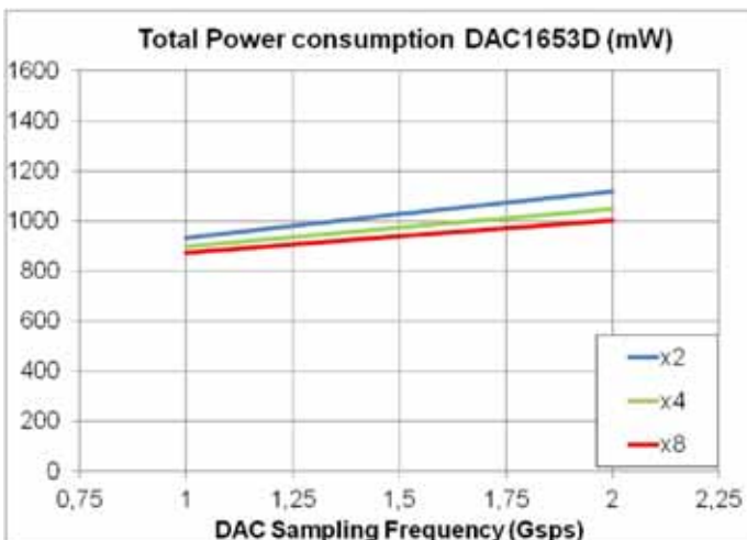
Fig 28. Total Power consumption DAC1653D (mW) depending of the DAC sampling frequency and the interpolation factor (all digital features off)
