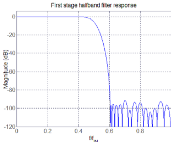
Fig 43. First stage half-band filter response (used in ×2, ×4, and ×8 interpolation)
