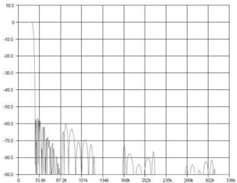
Figure 13: DAC Pass Band Suppression (Audio Mode, 48 kHz)
