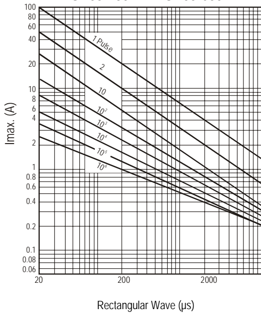
ROV05-820K – ROV05-471K
