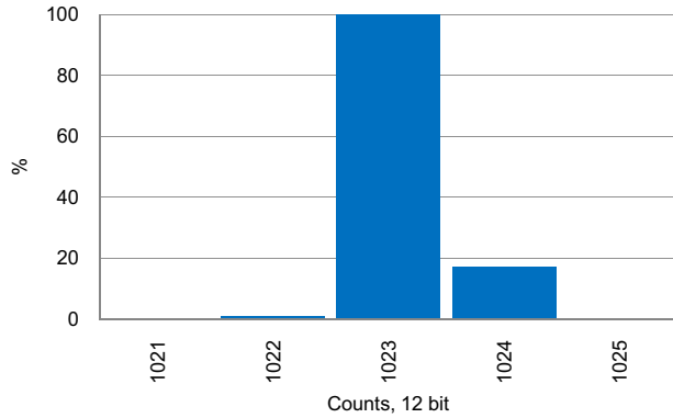
Figure 11-37. SAR ADC Noise Histogram, 100 ksp/s, Internal Reference No Bypass
