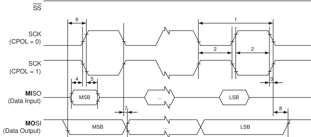
Figure 35-3. SPI timing Requirements (Master Mode)
