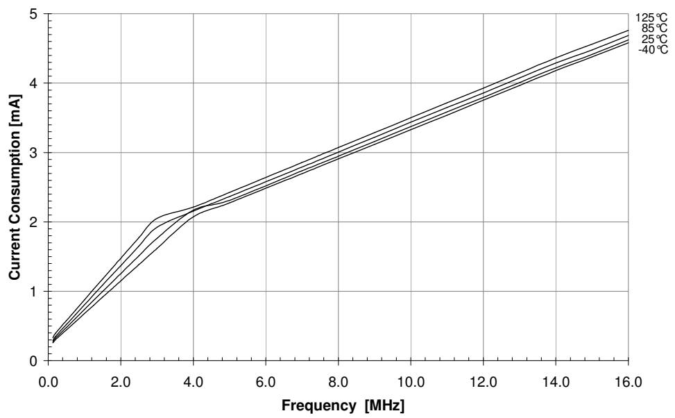
Figure 36-10. Active Supply Current vs. Frequency ( V_{DD} = 3.0\text{V} , PRR0/1 = 0x00/0x00 )
