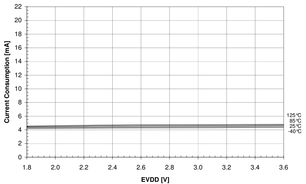
Figure 36-14. TRXOFF state supply current vs V_{\text{DD}}
