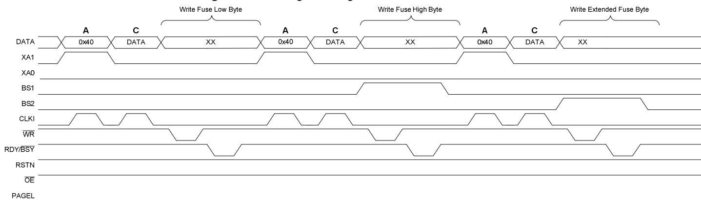
Figure 31-8. Programming the Fuses Waveforms
