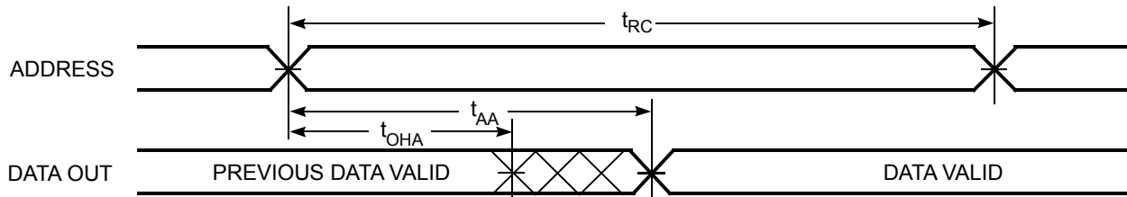
Figure 4. Read Cycle 1: Address Transition Controlled [21, 22]
