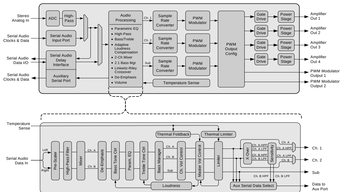
Figure 14. Digital Signal Flow
