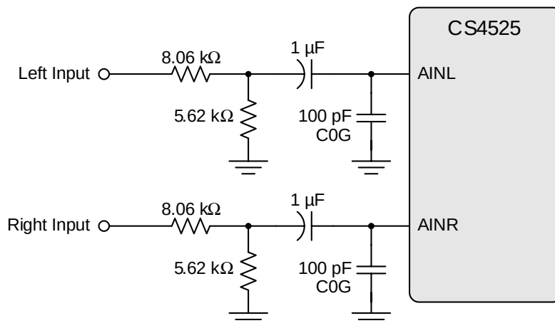
Figure 29. Recommended 2 V RMS Input Filter
