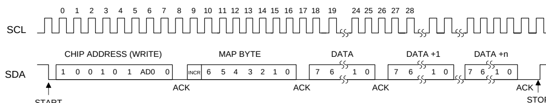
Figure 33. Control Port Timing, I 2 C Write
