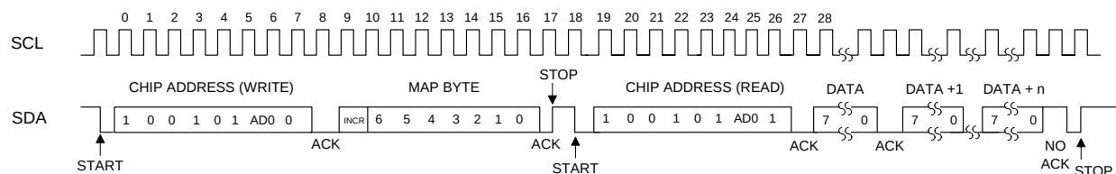
Figure 34. Control Port Timing, I 2 C Read
