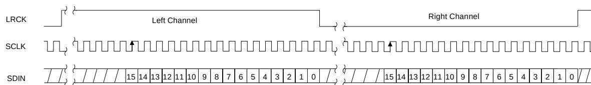
Figure 32. Right-Justified Serial Audio Formats
