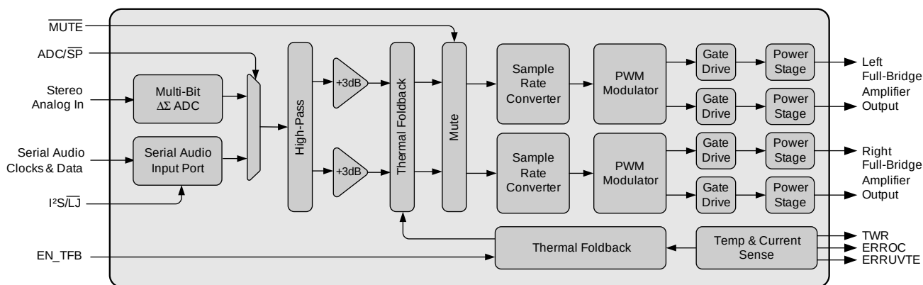
Figure 24. Hardware Mode Digital Signal Flow
