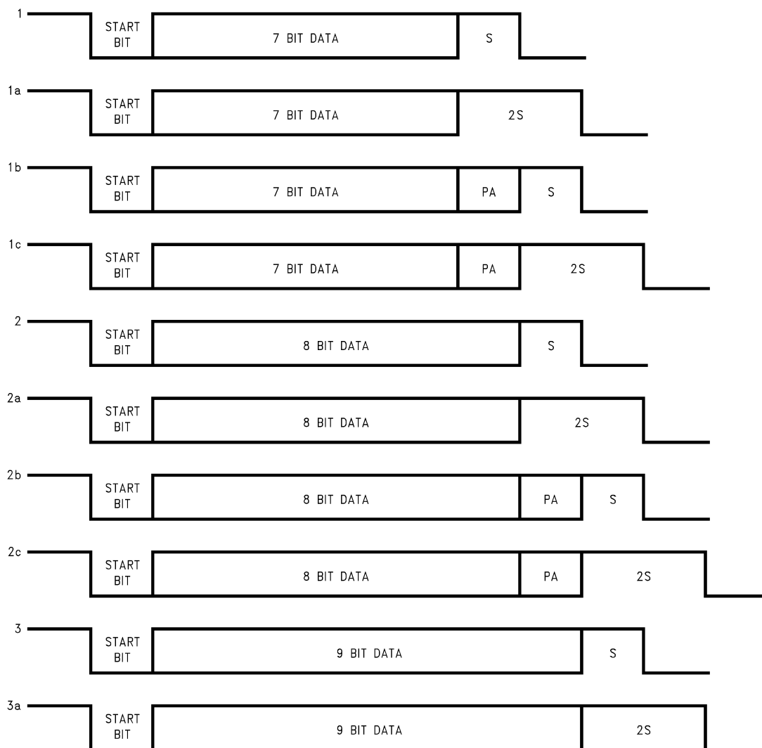
Figure 5-17. Framing Formats
