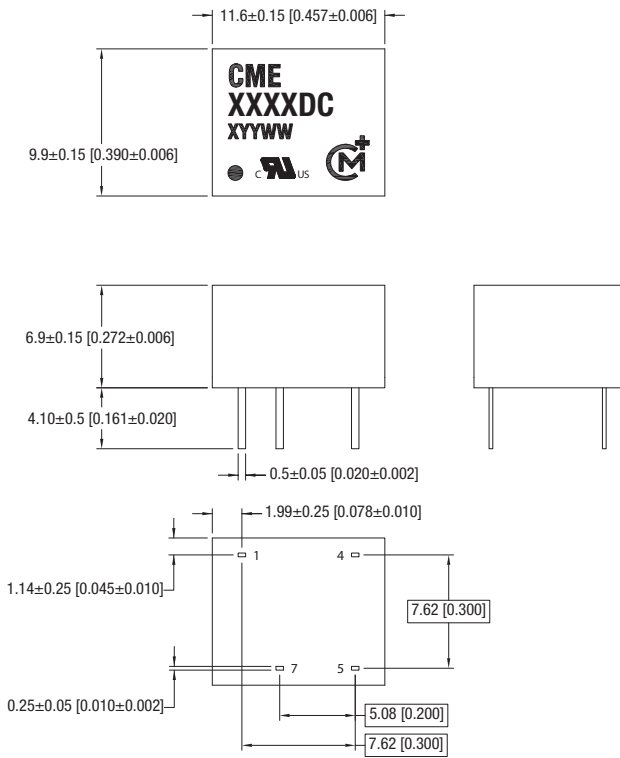
3C Package
