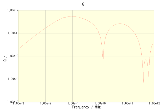
CLF6045T-471M-CA
