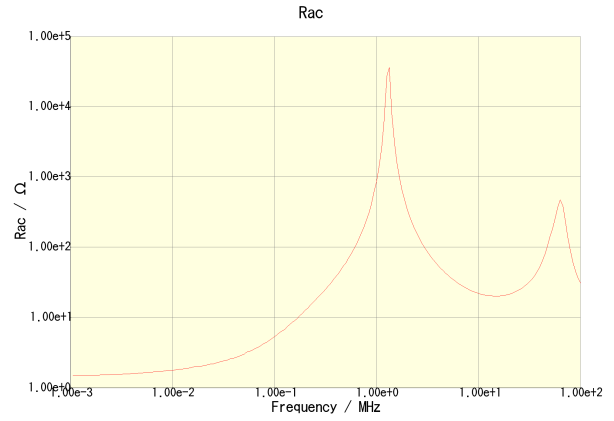
CLF6045T-471M-CA
