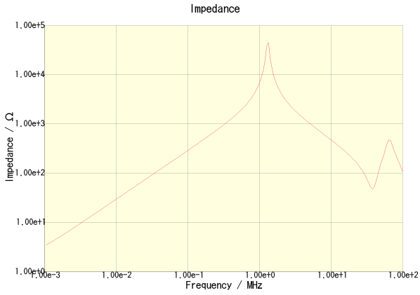
CLF6045T-471M-CA
