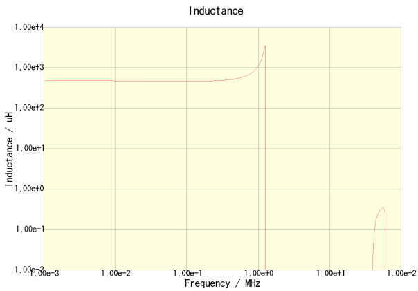
CLF6045T-471M-CA
