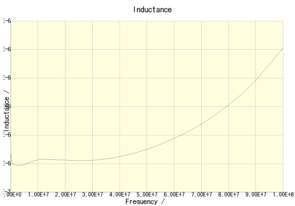
CLF12555T-1R0N-CA
