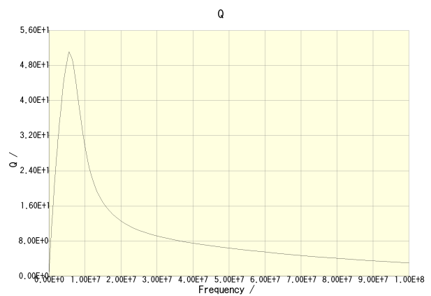
CLF12555T-1R0N-CA
