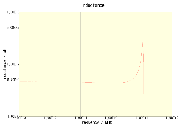
CLF10040T-470M-CA
