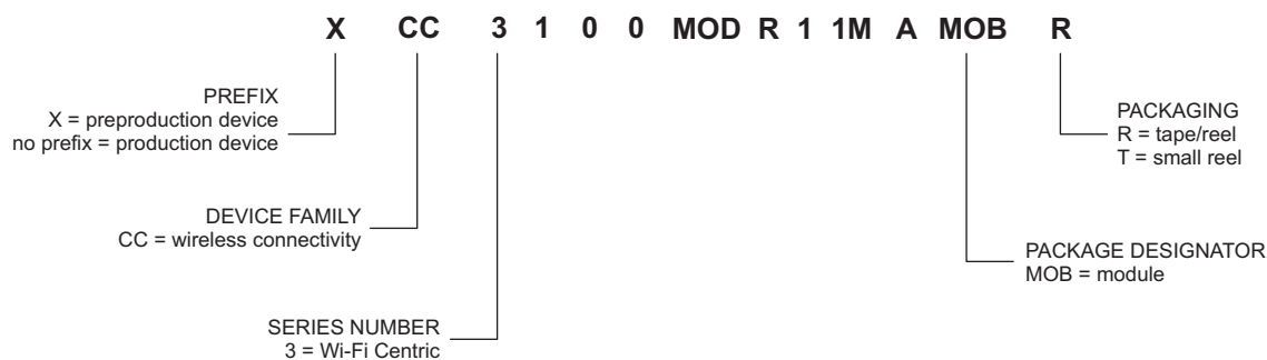
Figure 8-1. CC3100MOD Device Nomenclature
