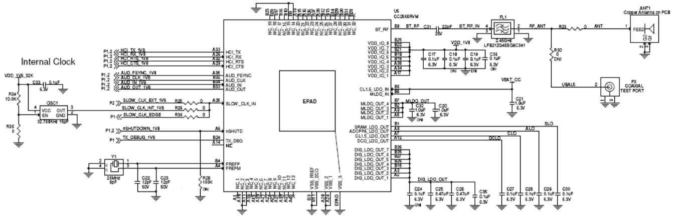
Figure 2. Reference Design Schematics
