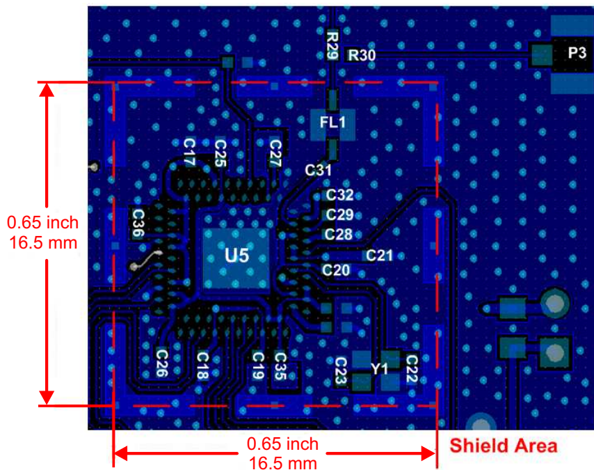
Figure 3. Component Placement
