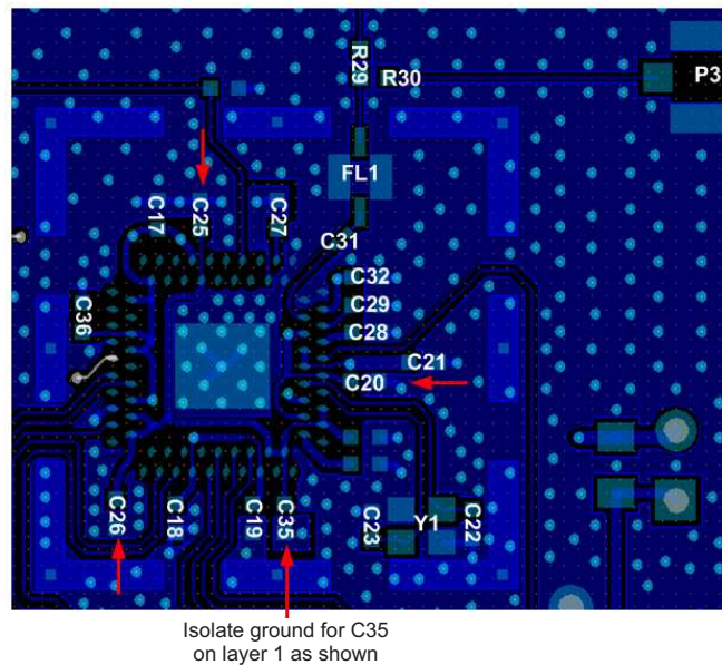
Figure 4. LDO Capacitor Placement
