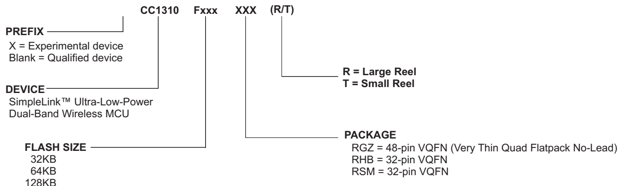
Figure 8-1. Device Nomenclature
