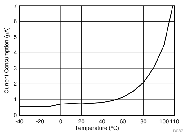
Figure 5-5. Standby MCU Current Consumption, 32-kHz Clock, RAM and MCU Retention
