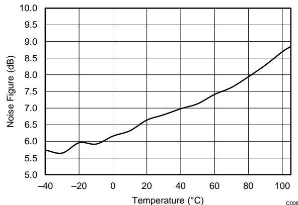
Figure 4-8. Noise Figure with 2-MHz Bandwidth vs Temperature
