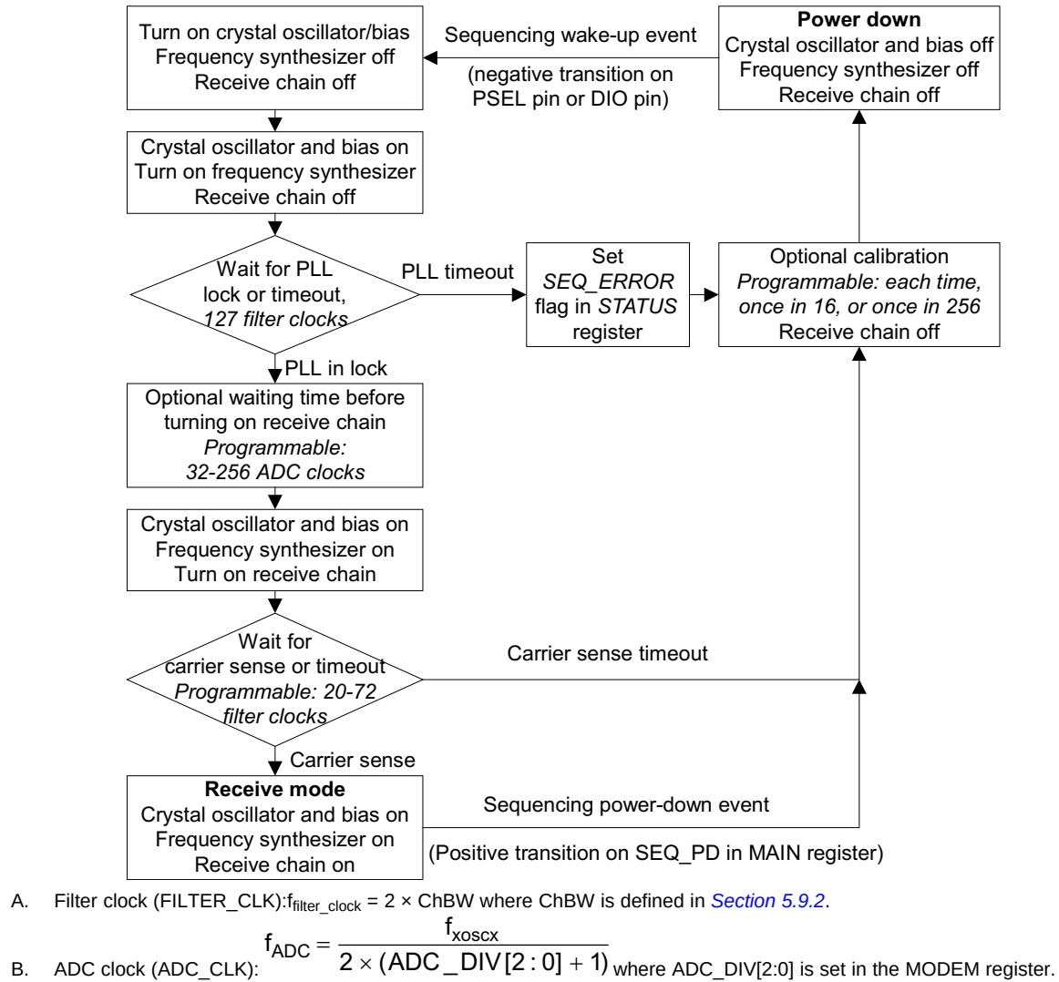
Figure 5-18. Automatic Power-Up Sequencing Flow Chart
