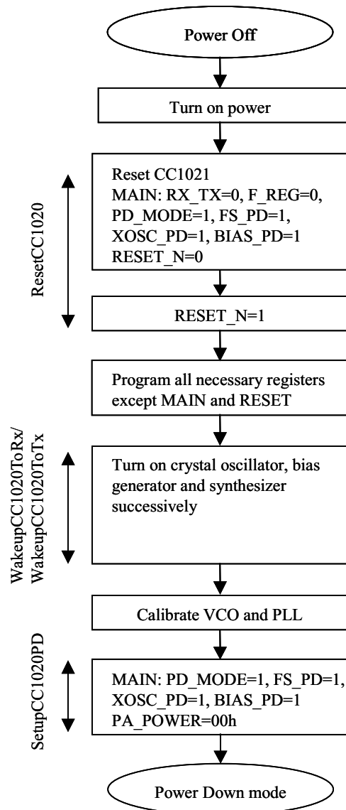
Figure 5-27. Initializing Sequence
