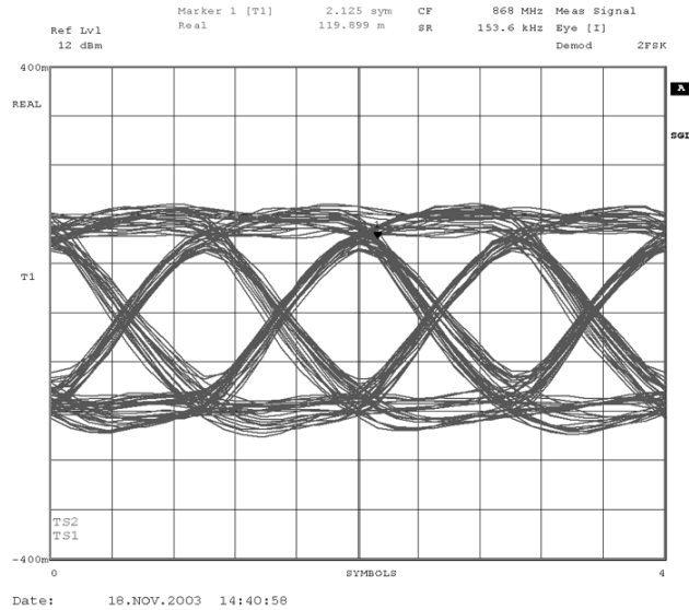
Figure 5-19. GFSK Eye Diagram. 153.6 kBaud, NRZ, \pm 79.2 kHz Frequency Deviation.
