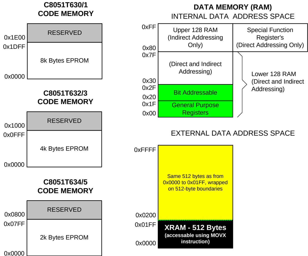
Figure 13.1. Memory Map
