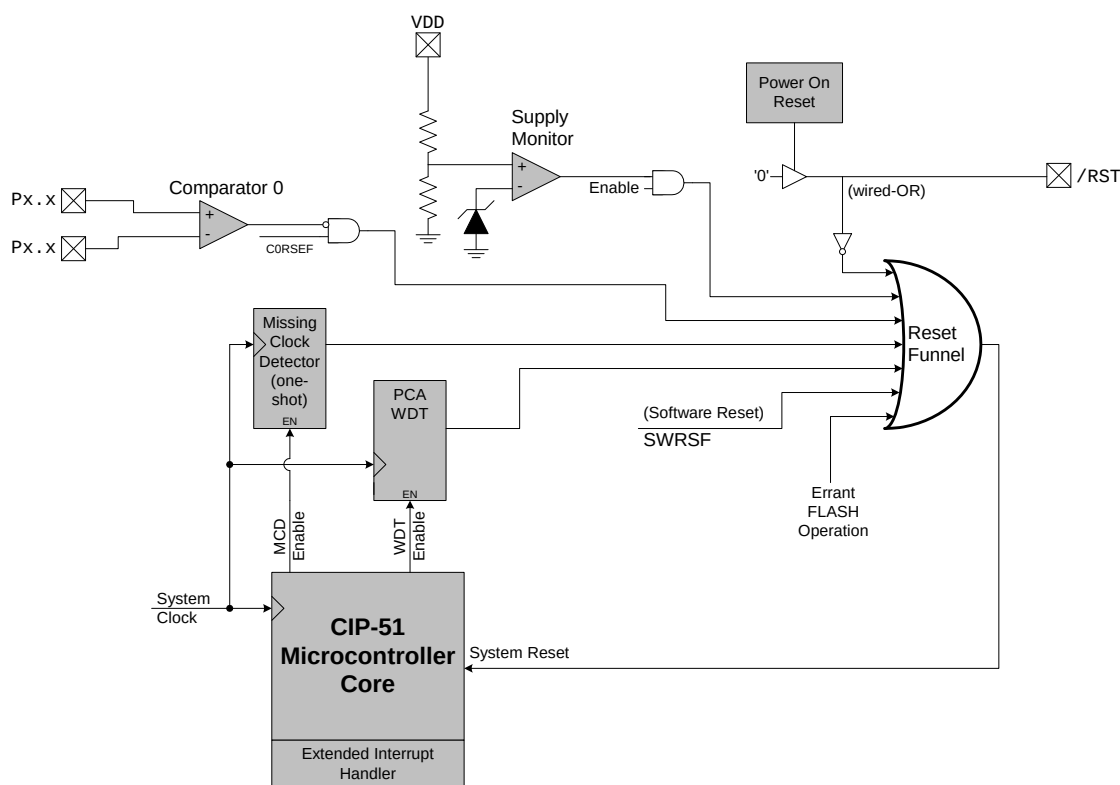
Figure 9.1. Reset Sources
